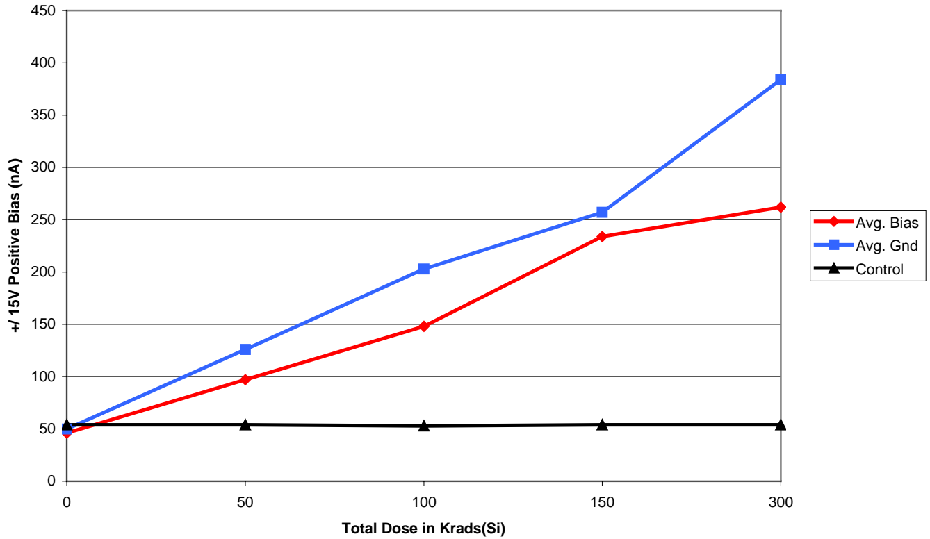
+/- 15V Positive Input Bias vs. Total Dose
