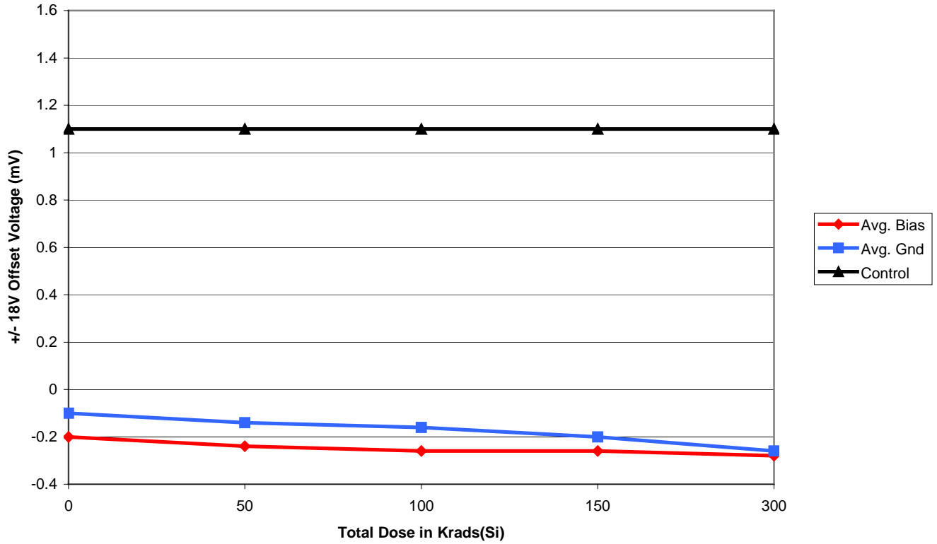
+/- 18V Offset Voltage vs. Total Dose
