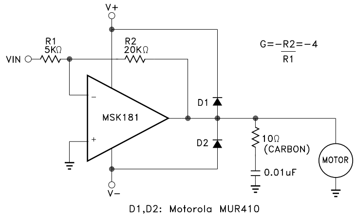
Figure 4 Motor Drive Circuit
